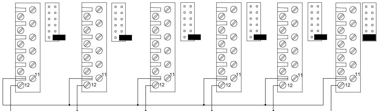
Figure 4. Connecting units together for sync guard.
