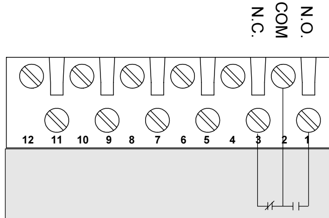
Figure 3. Connections for shorted SCR detection relay.
