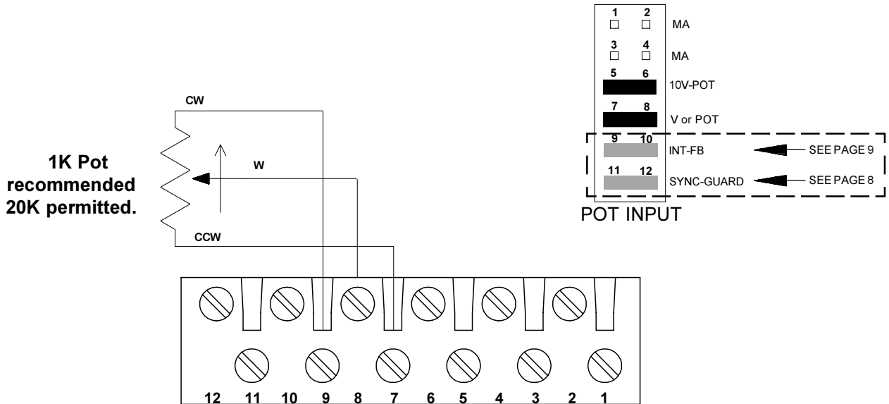
Figure 6. Connections for using a pot as a command control.
