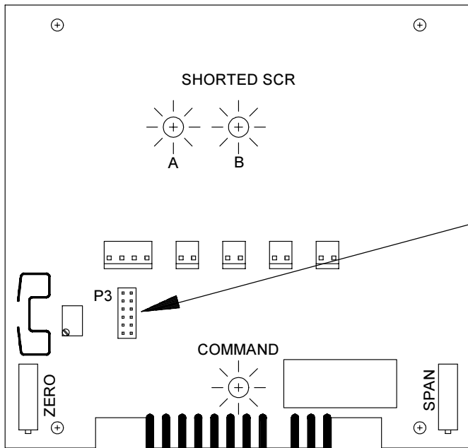
Figure 9. Jumper positions for Voltage inputs.
