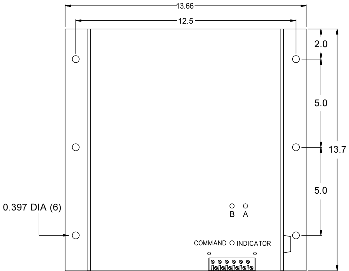
Figure 2. Mounting dimensions, Model 3037, 240 to 425 Amps. SEE PAGE 6 FOR FUSE ORIENTATION
