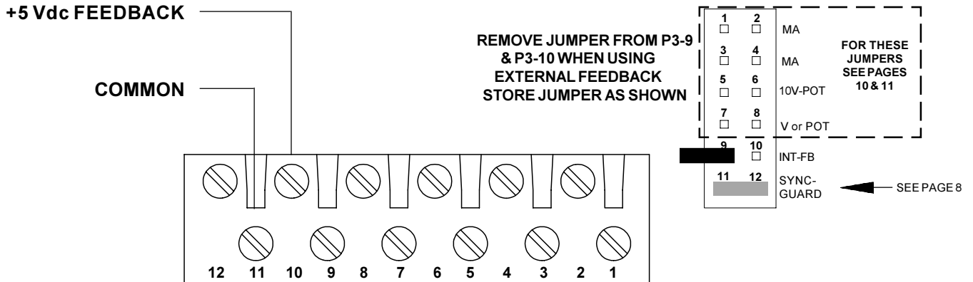
Figure 5. External feedback is a 0 to 5 Volts D.C. signal representing the variable to be controlled. For example; Power, Current, Voltage, ETC.
