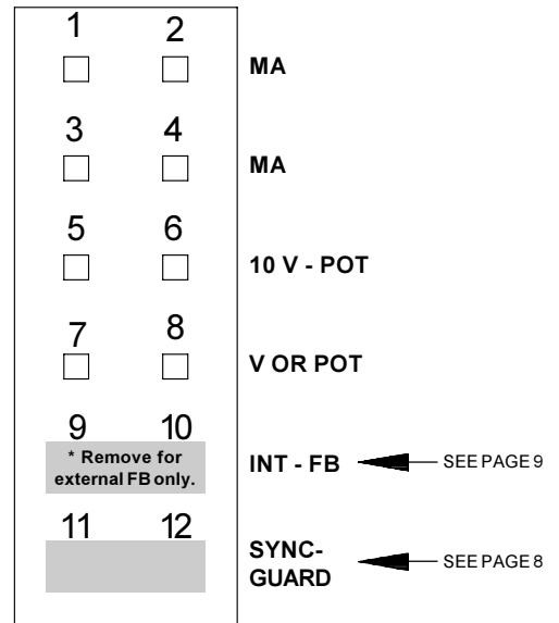
Figure 10. P3 jumper positions
