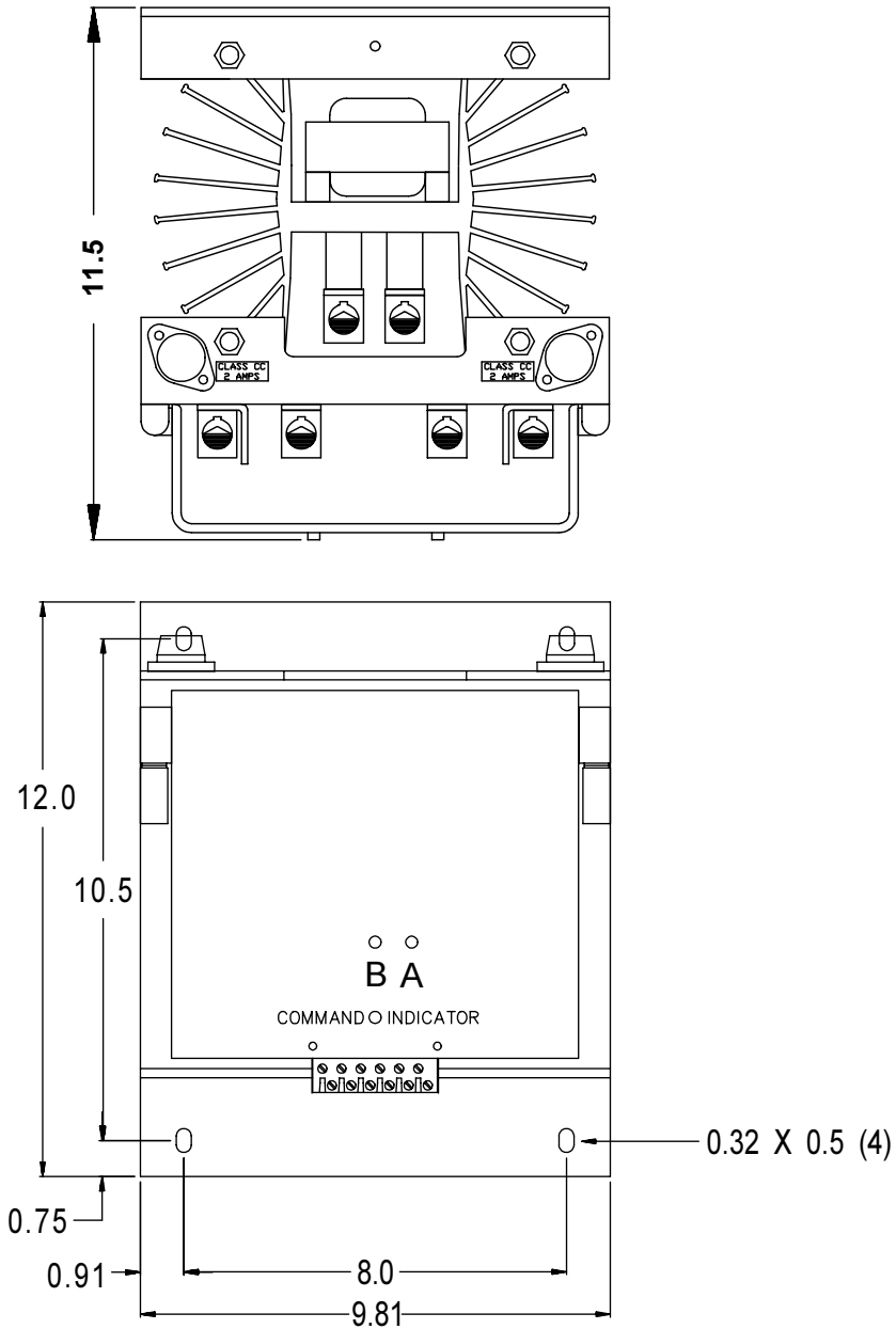
Figure 1. Mounting dimensions, Model 3037, 85, 145 and 175 Amps (145 & 175 Amp units have forced air cooling.)
