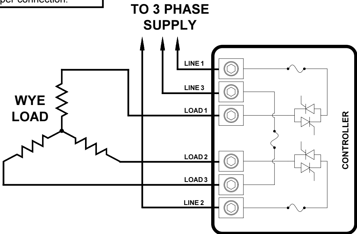
Figure 11. In-line power connections.
