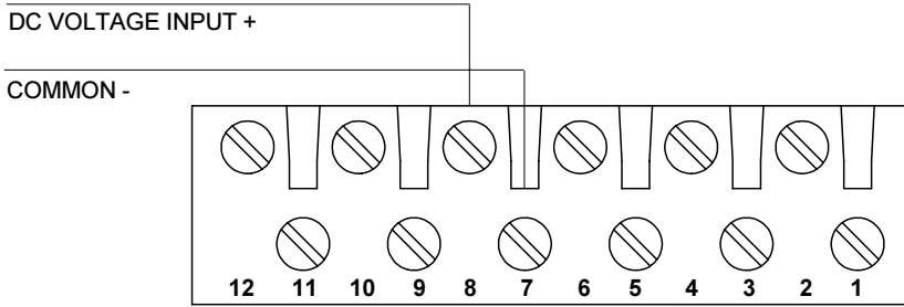
Figure 8. Connections for a voltage command signal.
